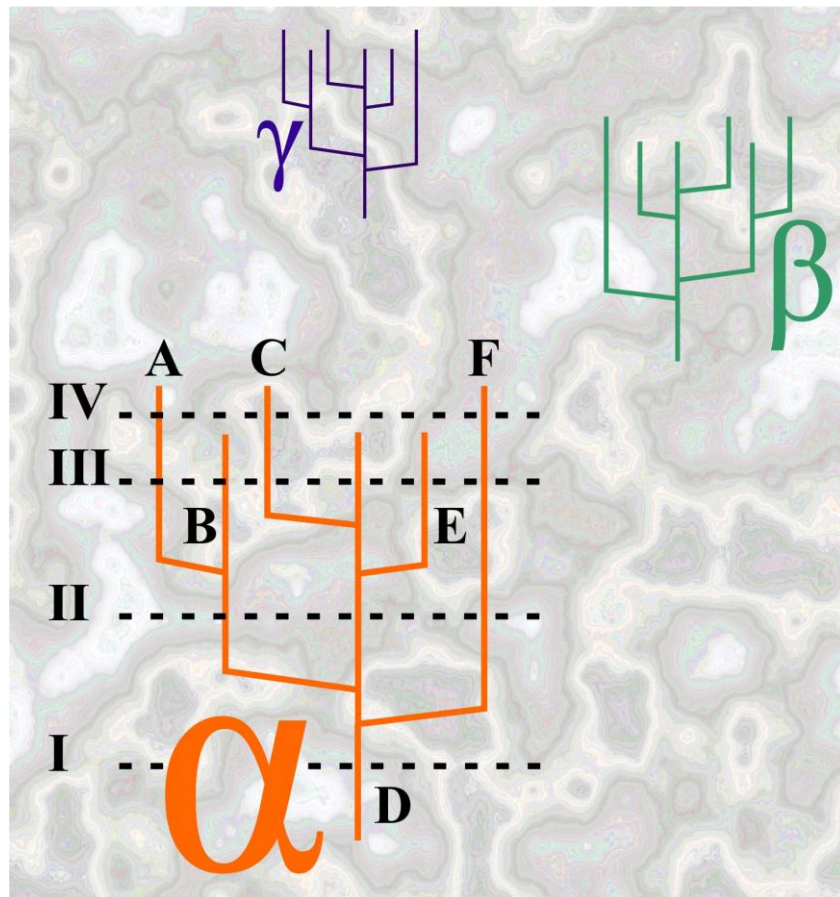
Fig. 4. Diachronic polymorphism. Schematic representation of Wasmann's concept of phylogenesis.
